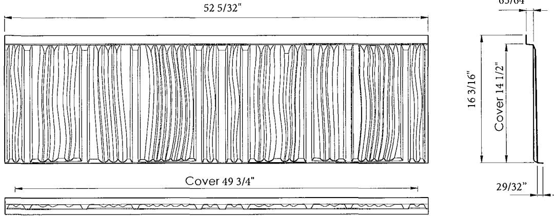
Figure 2.1 Tile Dimensions
