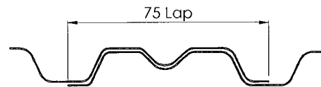
Figure 2.4 Lap Section
