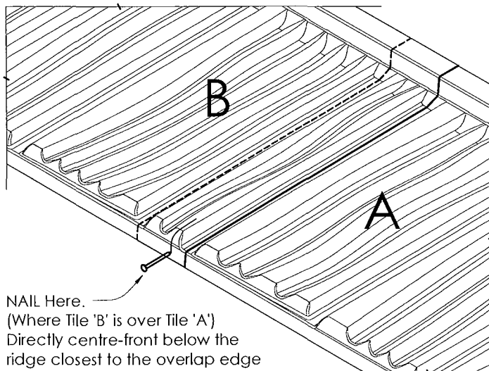
Figure 2.3 Overlap Detail
