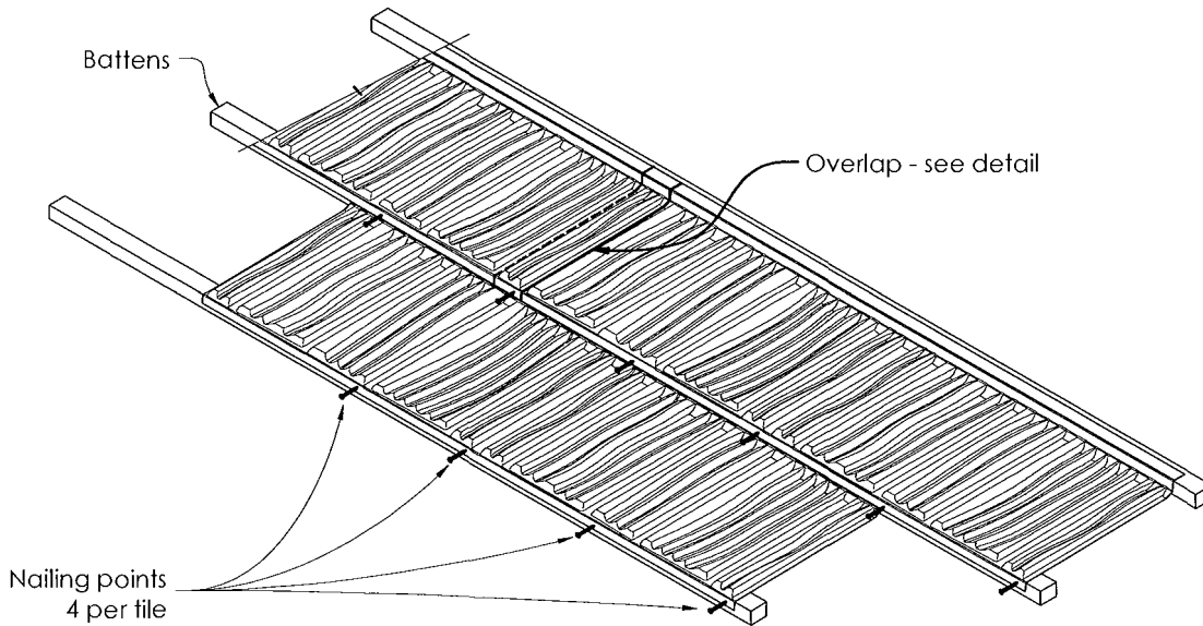
Figure 2.2 Nailing Detail
