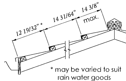
Figure 2.5 Batten Layout
